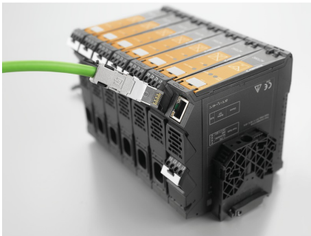
ACT20C station with gateway and current converters
