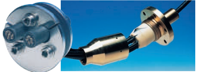
PHP pressure hull penetrator for submarines.
