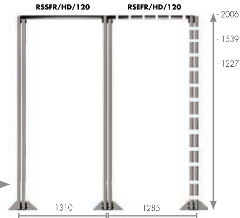
Frame Purchase Example: R5SFR/HD/120/1539
