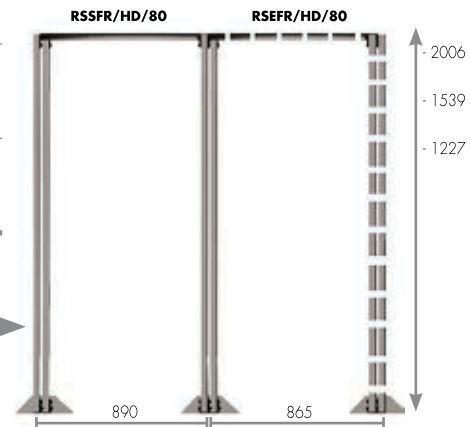
Frame Purchase Example: R55FR/HD/80/1539
