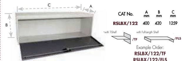
Lockable box for 12 Series shelving. Box and shelving construction: 0.9 and 1.1mm zinc annealed and powder coated.
