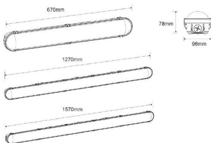
Dimension Diagram
